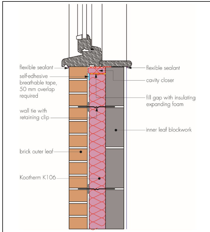
Figure 5 Reveal details — cavity closer
