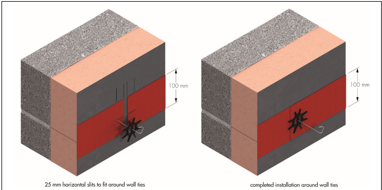
Figure 7 Self-adhesive breathable tape applied around wall tie penetrations
