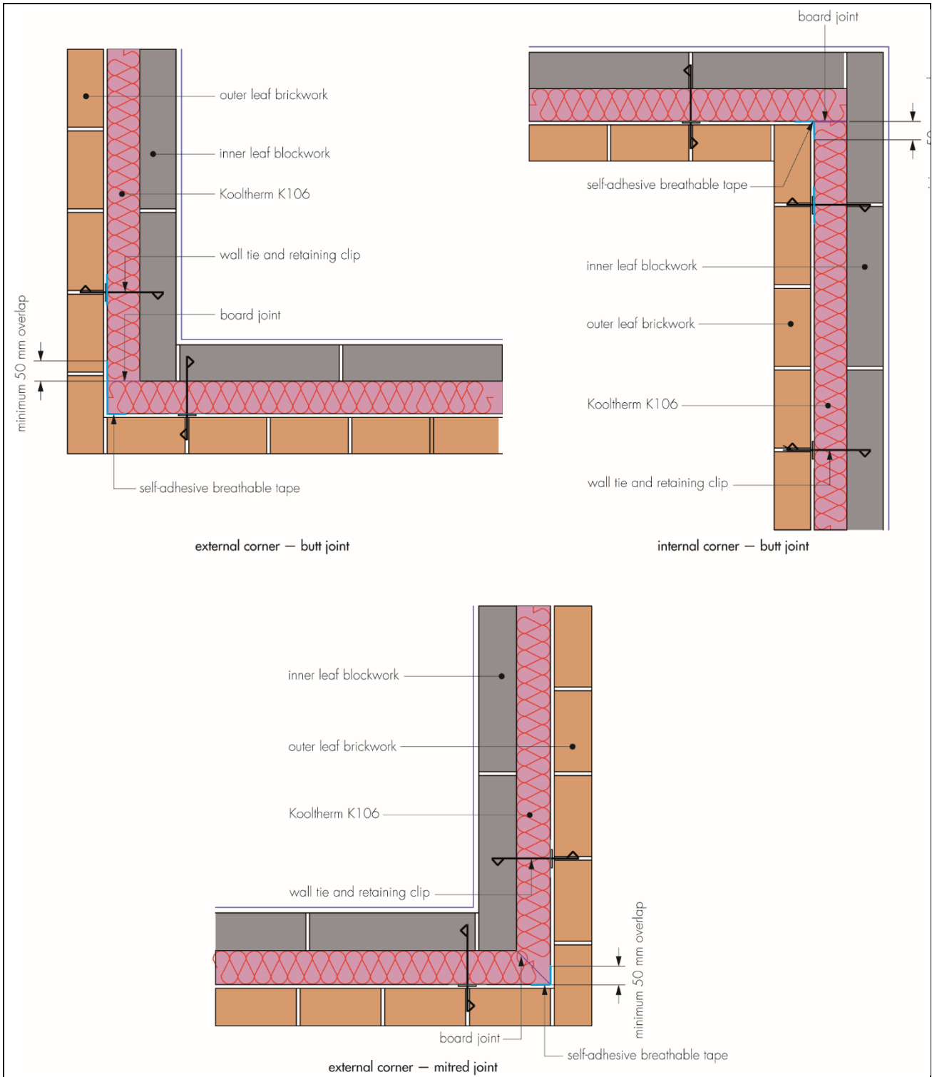
Figure 8 Corner details
